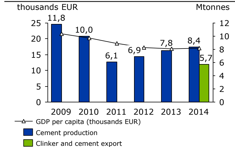
Greek cement production including exported clinker and GDP
