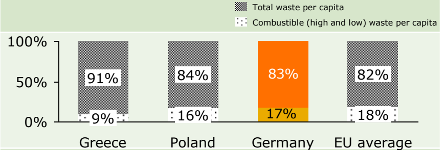
WtE capacity as share of combustible waste (2012)*
