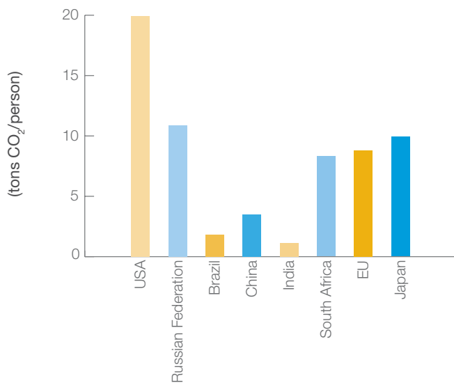
Annual GHG per Capita
