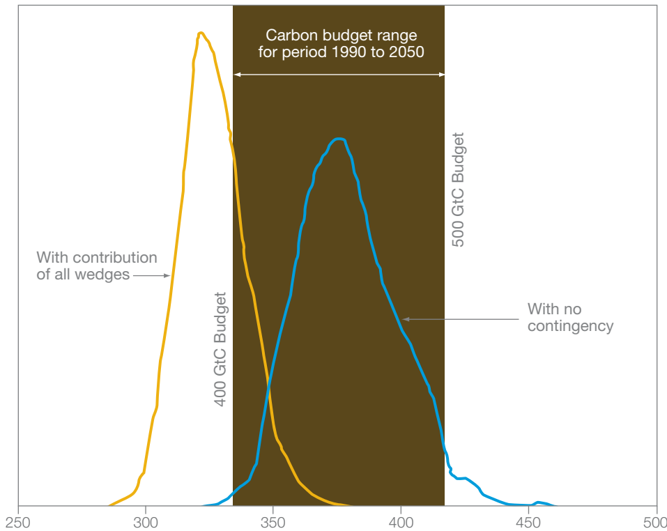
Figure 10. Probability distribution of carbon emissions staying within the 400GtC and 500GtC budgets for the period 1990-2050 in WWF’s Climate Solutions scenario. Note that the total budget is spent over the period 1990 to 2200; however, this figure considers the component of the budget in the period to 2050. The 400GtC budget to 2200 corresponds to a budget of 340GtC to 2050, and the 500GtC budget to 2200 corresponds to a budget of 415GtC to 2050. The yellow and blue lines represent the outputs of multiple runs of the Monte Carlo model (as number of hits). The yellow and blue lines correspond to the lower and upper limits (respectively) of the red band in Figure 8.
