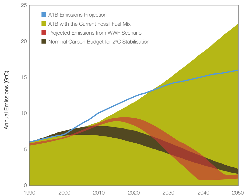
Figure 6. Emissions in the WWF Climate Solutions Model. The diagram shows the range of emissions (red bands) in the scenario presented in this paper. The lower limit of the red band shows the technical potential of emissions reduction if all wedges are fully implemented, and the whole “fossil fuel with CCS” wedge (yellow in Figure 4) comprises plants burning gas (which has lower carbon intensity). Emissions follow the upper limit line if about 80% of the potential is achieved and the “fossil fuel with CCS” wedge is made up of (higher carbon intensity) coal plants. Placed against the nominal carbon budget curve (brown), it is clear that the overall emissions to 2050 of the lower trajectory fall within the total emissions indicated by the upper limit of the budget range (assuming that deforestation is successfully brought under control). Any failure of efforts to halt deforestation (reducing the budget available for energy emissions to the lower limit of the brown band) will reduce the chances of staying within the overall emissions budget, especially if failures or delays in the implementation of solution wedges drive the emissions curve towards the upper limit of the red band. These curves are set against a backdrop (green) of the emissions that would occur if the IPCC’s A1B energy scenario were supplied with the current fossil-fuel mix (i.e., at about 0.02GtC/EJ). Also shown is the projected emissions curve for the A1B reference scenario which reaches annual emissions of 16GtC in 2050. The results of the modelling show that, although the point at which global emissions start to decline may not occur until 2015-2020, there is potential to drive deep cuts quickly once the industrial momentum behind transition is underway.
