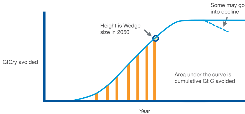
Figure 3. Emissions abated as a new technology grows.
