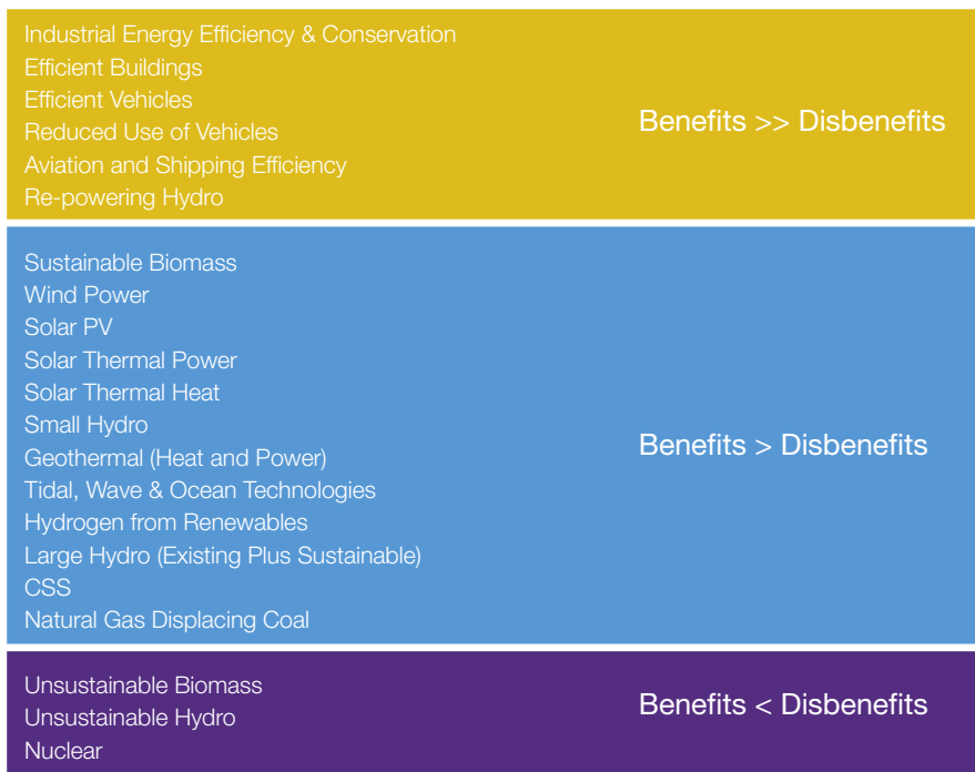
Figure 2. WWF grouping of climate solutions technologies based on environmental, social, and economic criteria.
